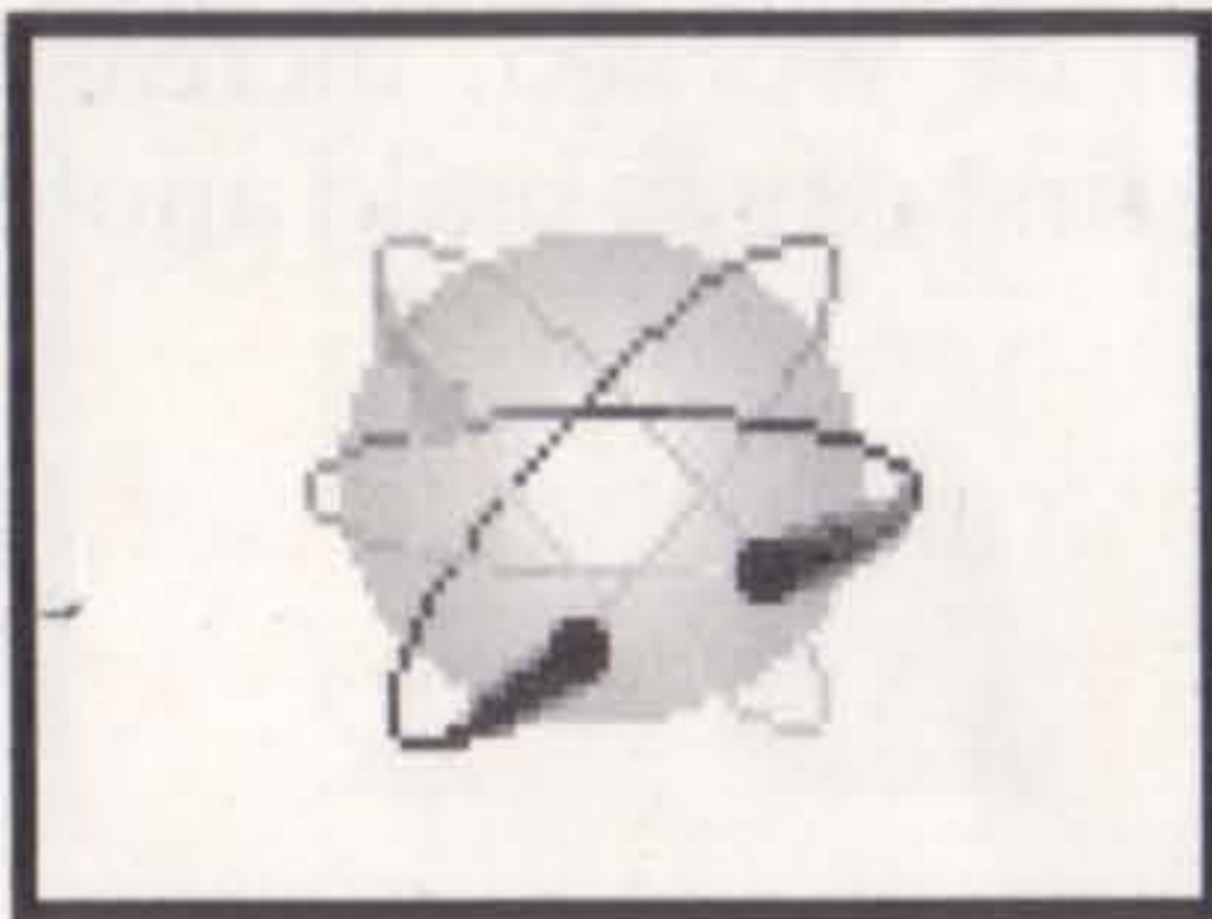
Atomic Theory (Theory of Gravity & Physics)
