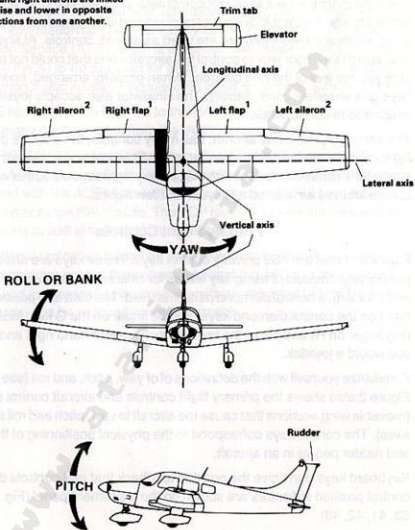
a) Control surfaces and rotational axes
