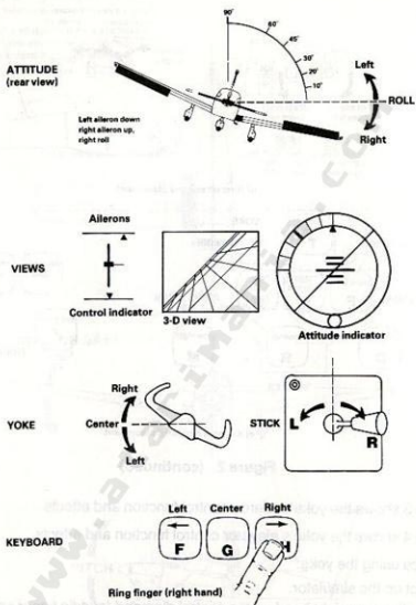
Figure 3. Ailerons – Controls and Effects
