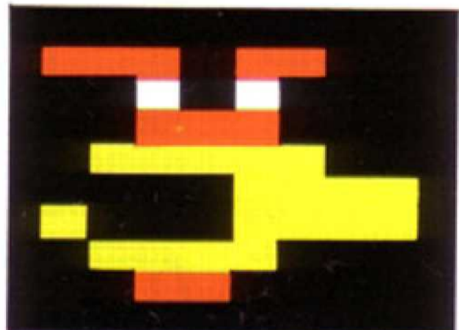
4. NASTROIDS
