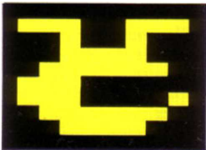
3. PARASOIDS
