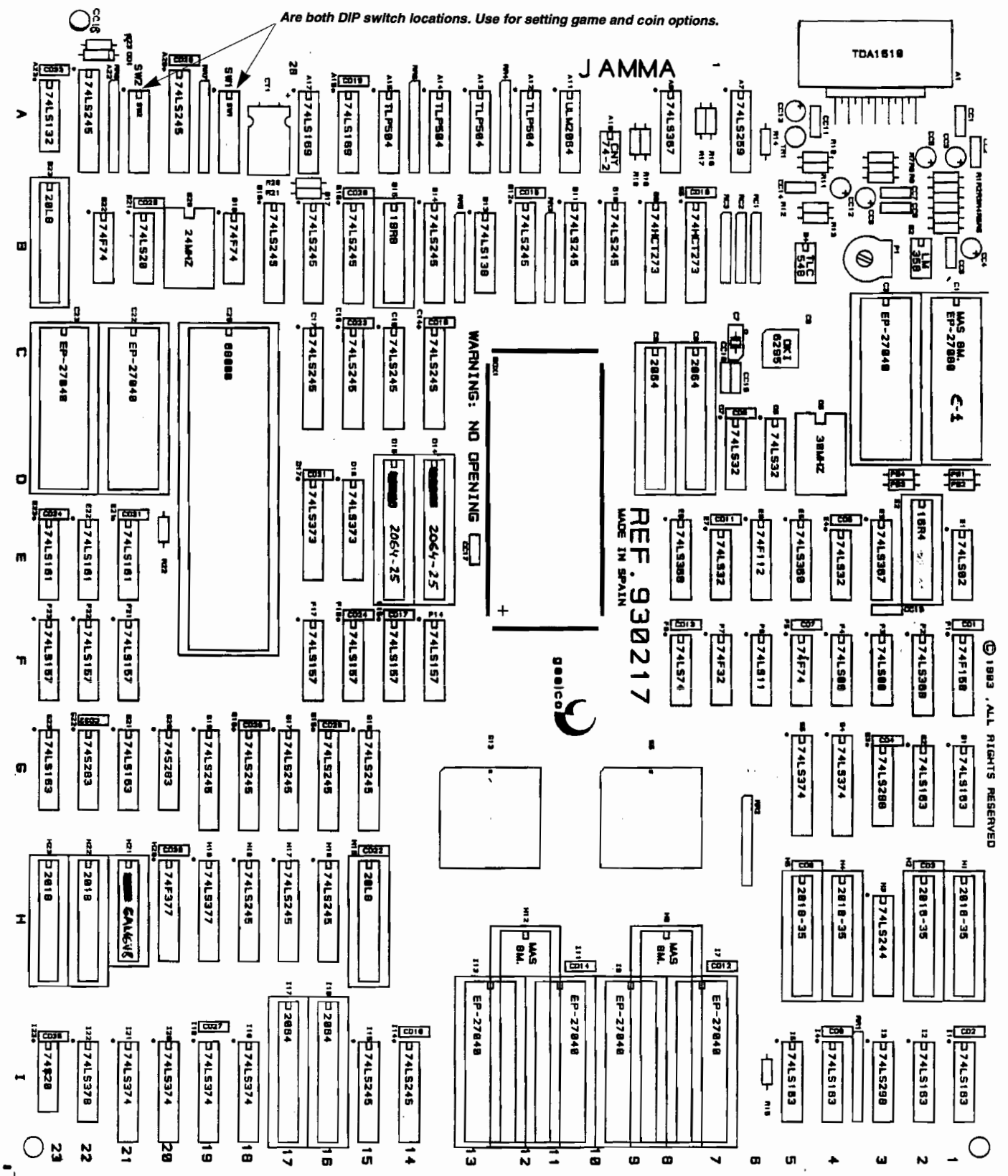
Figure 3-5 World Rally Game PCB Assembly 155035-001
