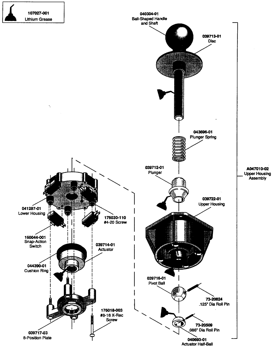
Figure 4-2 Microswitch Joystick Assembly A040933-03 B
