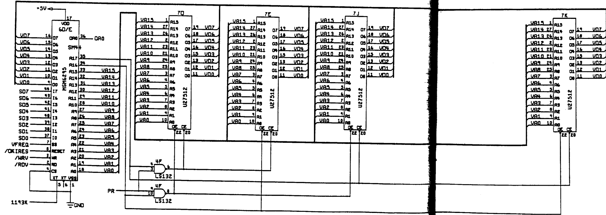
Figure 5-2 Skull & Crossbones JSA Audio II PCB Assembly Schematic Diagram, Sheet 2 of 3
