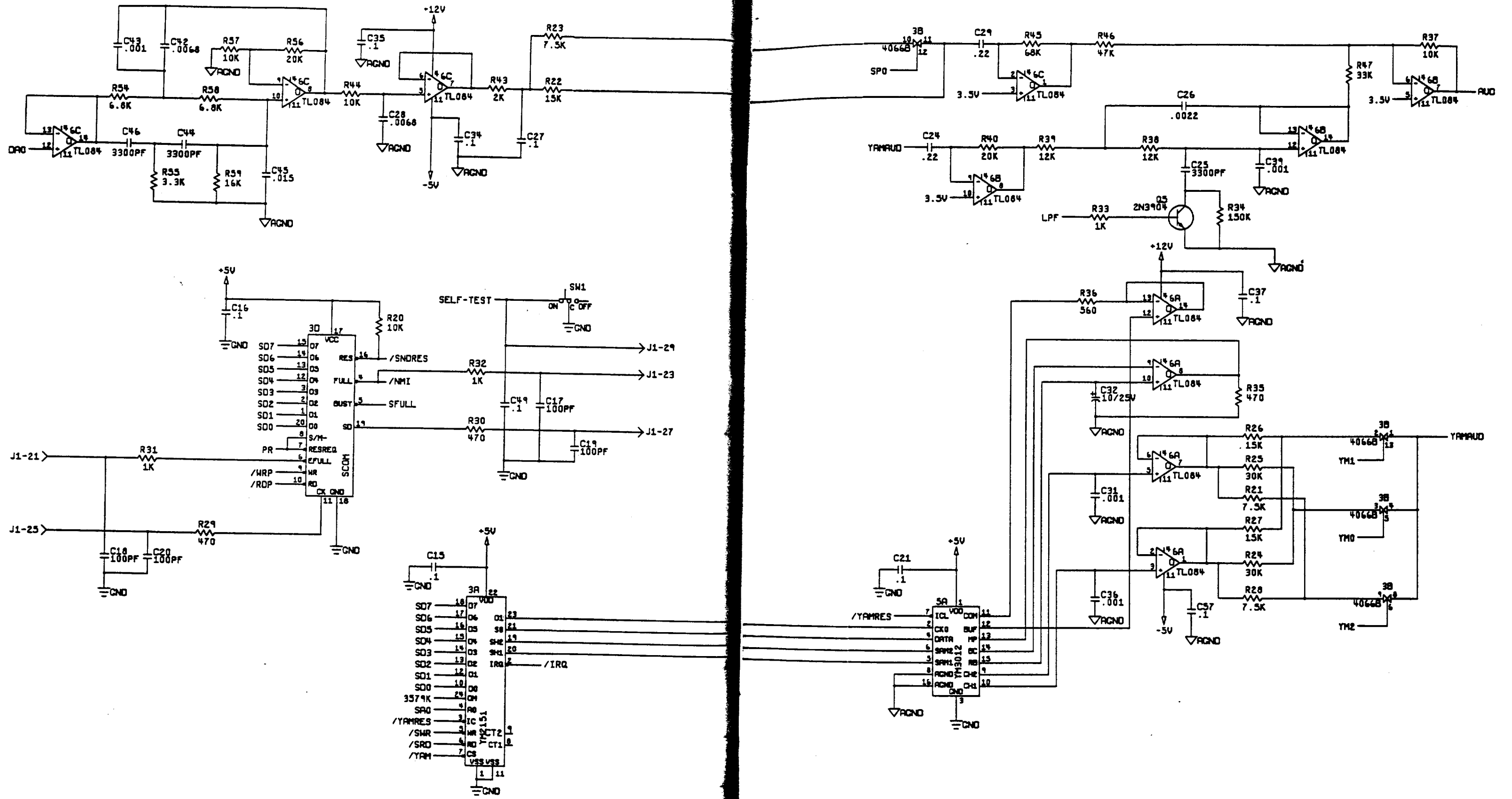
Figure 5-2 Skull & Crossbones JSA Audio II PCB Assembly Schematic Diagram, Sheet 3 of 3 046487-01 D
